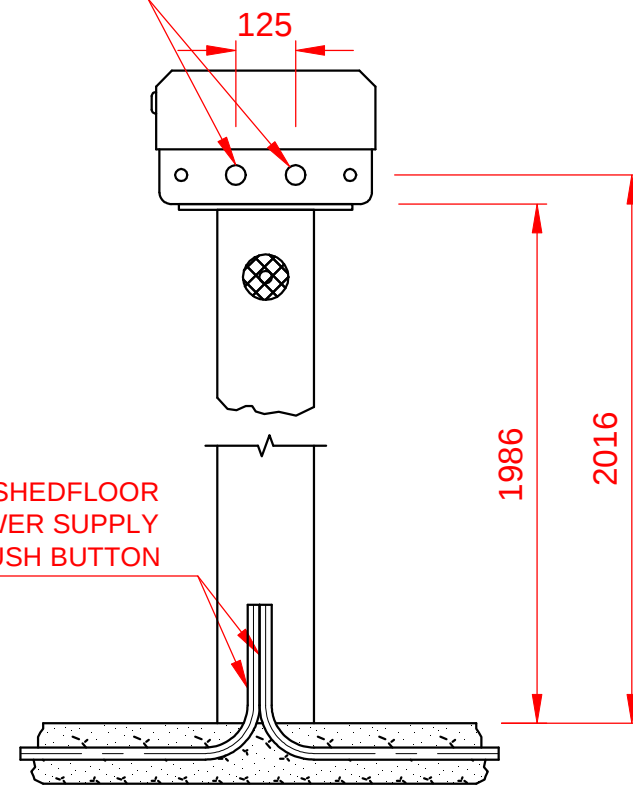
TURNSTILE SIDE ELEVATION
